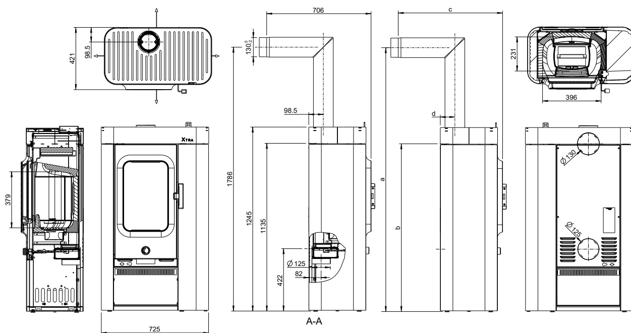
Fig. 2: Dimensions, Xtra incl. (option)
