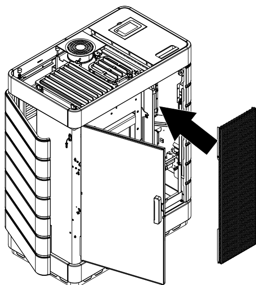
Fig. 63: Poser l'habillage
