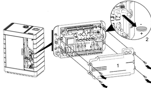
Fig. 88: Changing the storage battery
