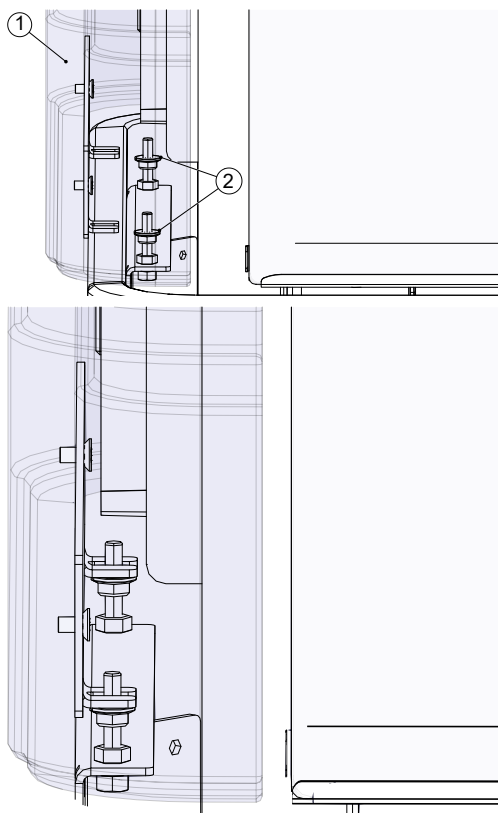
Fig. 25: Attaching the side cladding
