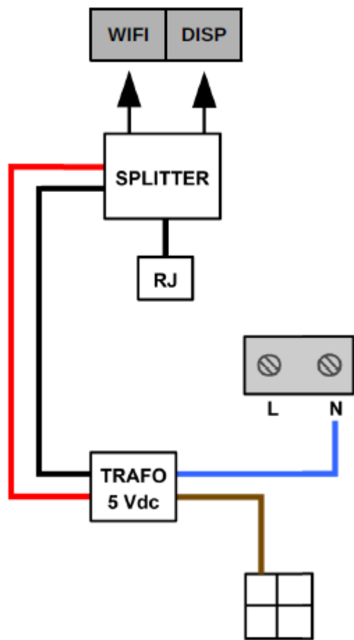
Electric connection diagram, detailed - data cable splitter
