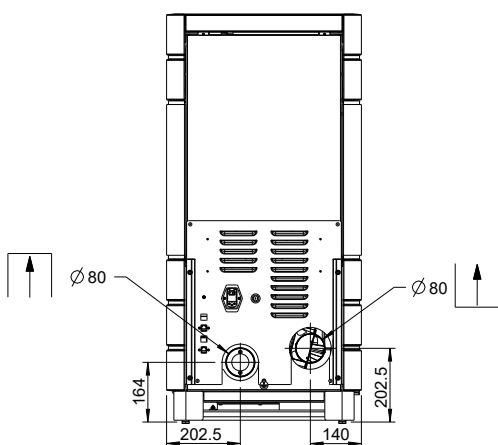
Fig. 28: Dimensions
