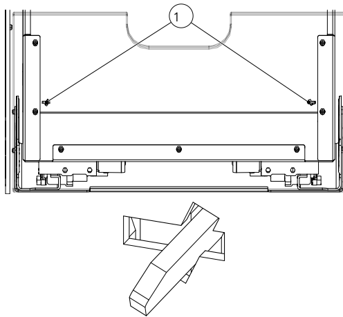
Abb. 27: Fixierzapfen
