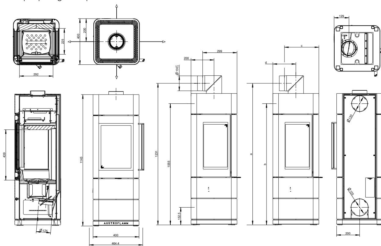
Fig. 1: Dimensions Ivy
