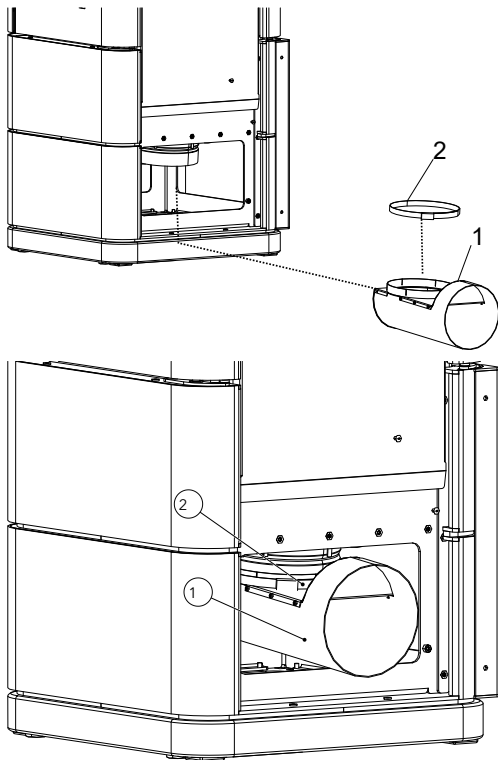
Abb. 24: Zuluftadapter montieren
