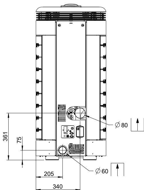
Fig. 22: Dimensions
