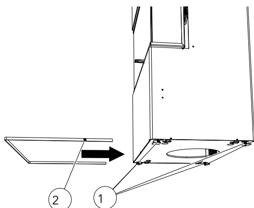
Fig. 16: Installer le joint creux
