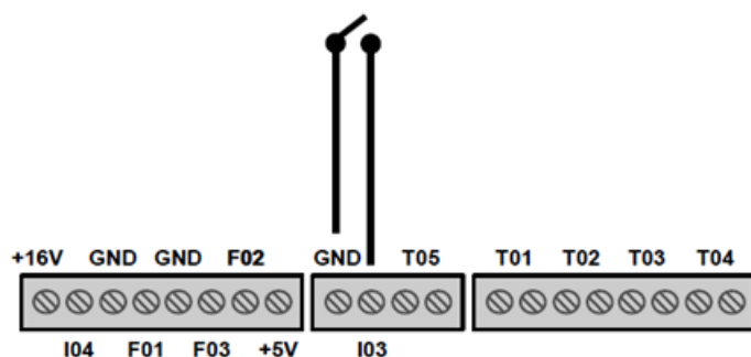
Fig. 17: Thermostat externe
