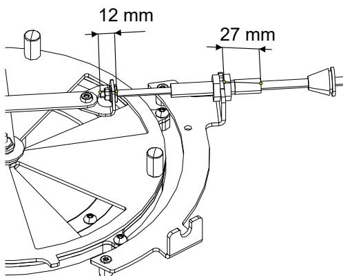
Fig. 57: Raccorder le câble Bowden
