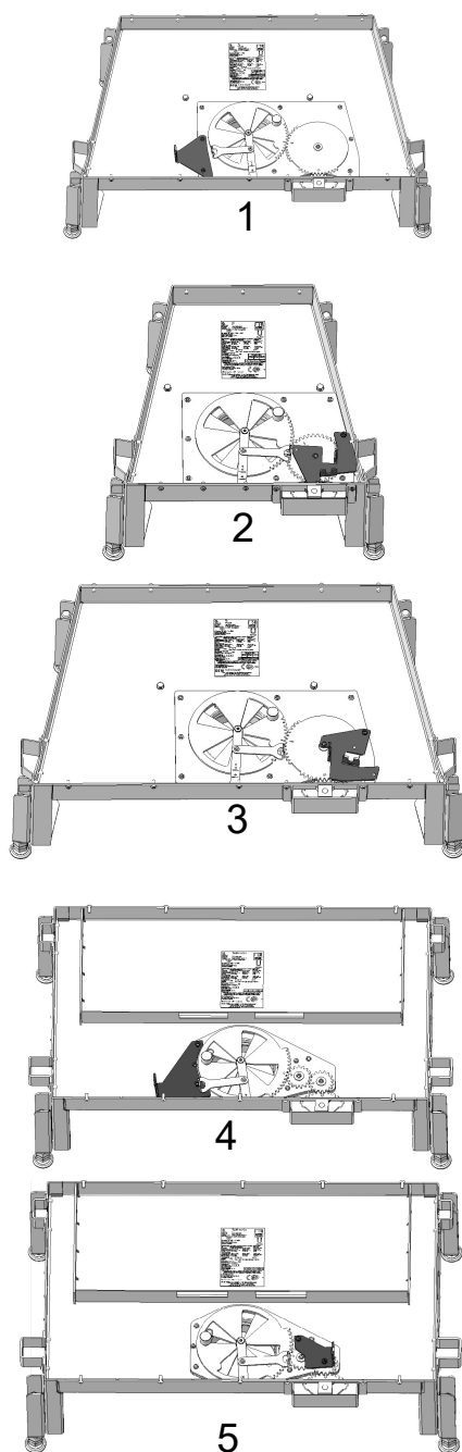
Fig. 51: Assembly situations
