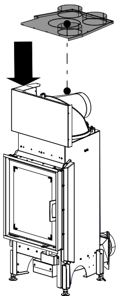
Fig. 67: Mounting the CV cover
