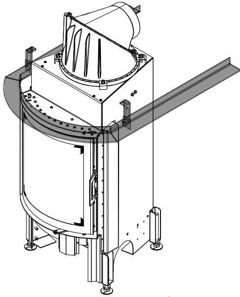
Fig. 96: Mounting the support frame
