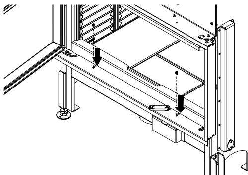
Fig. 90: Fixing the design frame at the bottom
