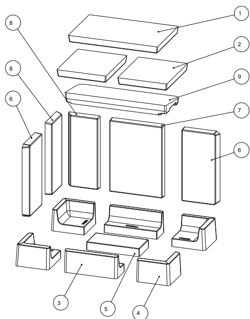
Fig. 23: Keramott 63x40x42
