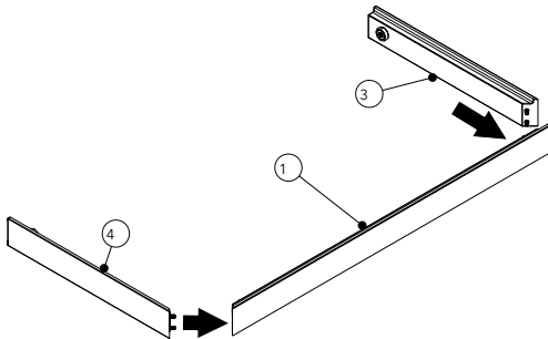
Fig. 9: Assemble the wooden base.
