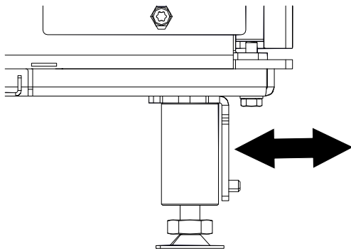
Fig. 8: Setting angle bracket
