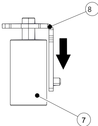
Fig. 3: Install the angle bracket and distance foot
