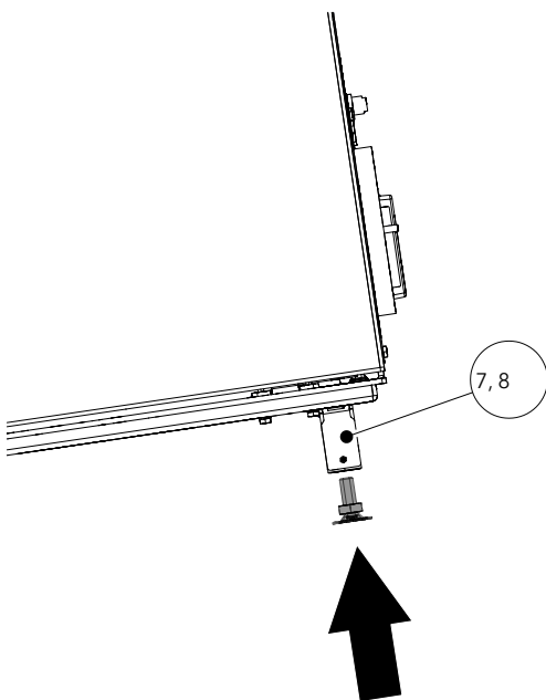
Fig. 7: Install the adjustable feet.
