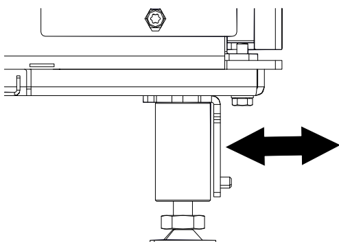
Fig. 5: Setting angle bracket
