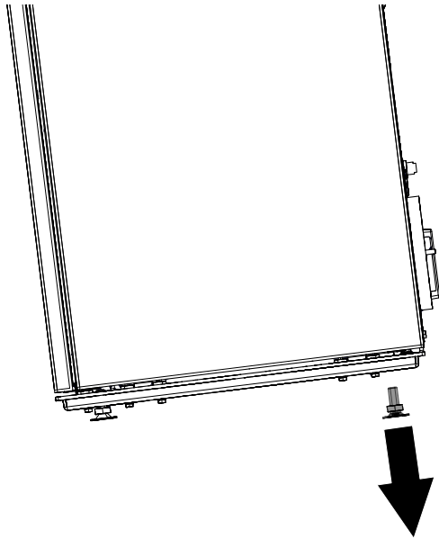
Fig. 2: Remove the adjustable feet.
