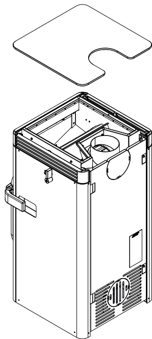
Fig. 1: Installing the hotplate
