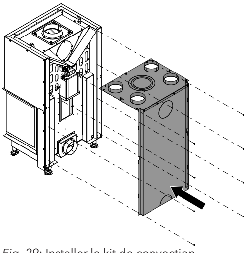
Fig. 29: Installer le kit de convection
