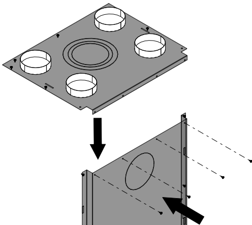
Fig. 28: Assembler le kit de convection
